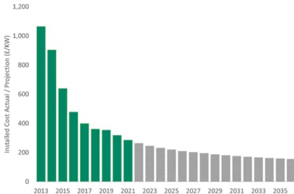
Figure 11-1: A projection of future battery component costs
