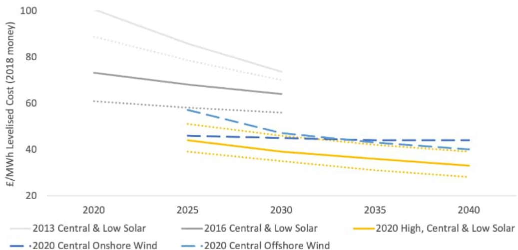
Figure 10-4: BEIS Cost of Generation. An evolution of Levelised Cost forecasts
