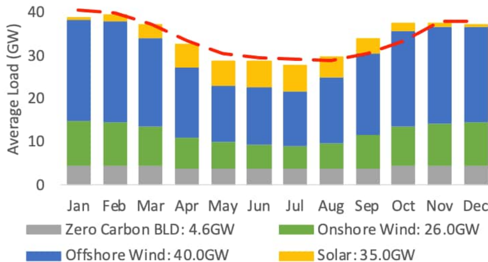
Figure 8-2: Deploying 35GW of large-scale solar alongside government offshore wind ambitions (40GW) meets anticipated seasonal demand levels
