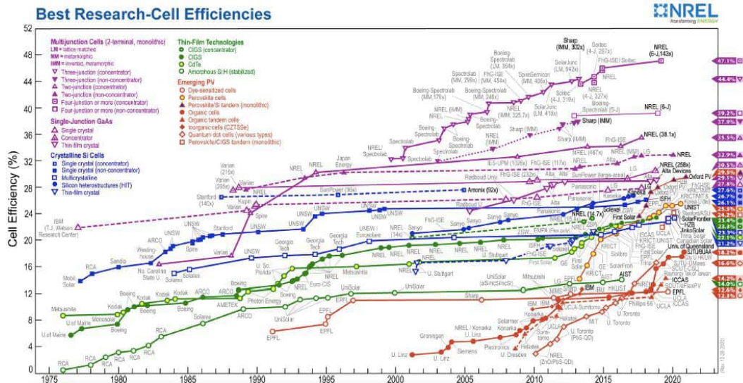
Figure 10-2: The efficiency of solar cell technology has increased year-on-year for decades
