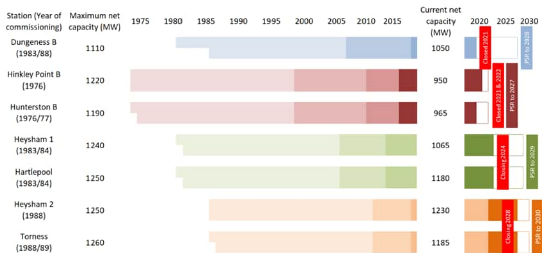
Figure 5-3: Generating capacities and announced closure dates for existing UK AGR stations
