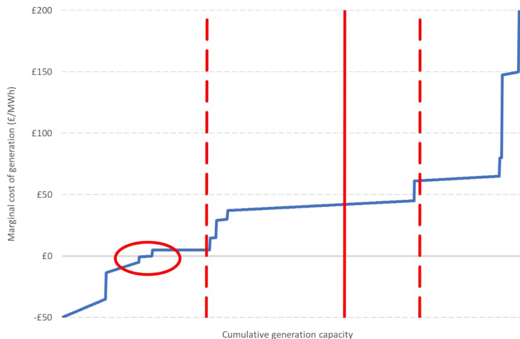
Figure 10-1: Representative marginal cost stack for the GB electricity system
