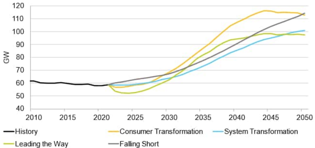
Figure 6-3: Future net peak electricity demand
