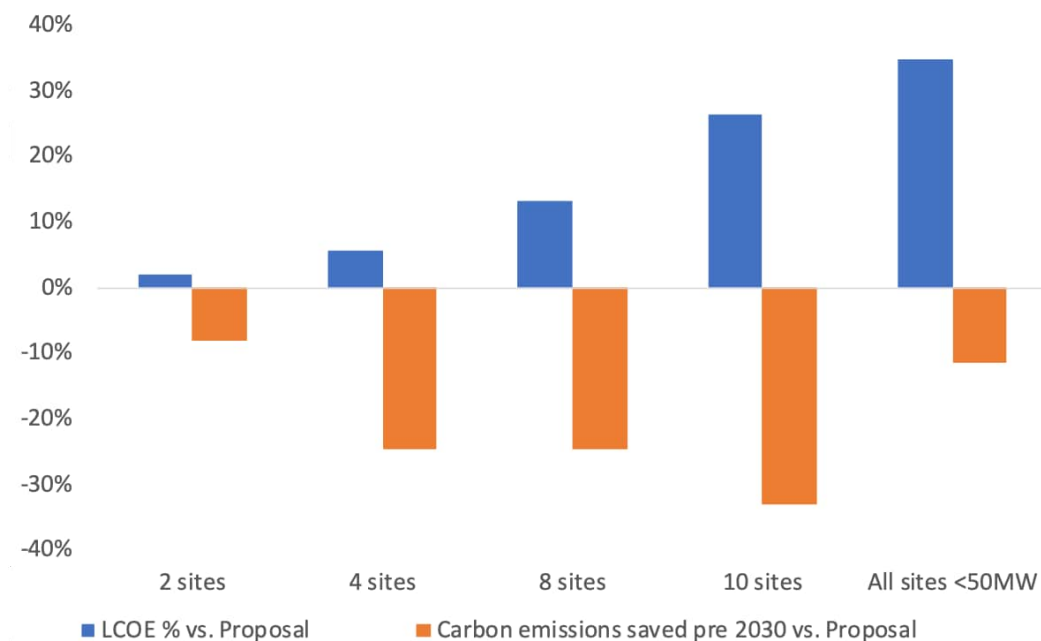
Figure 10-5: LCOE and carbon emissions savings at large-scale single-site solar, versus developing the same total capacity across multiple projects
